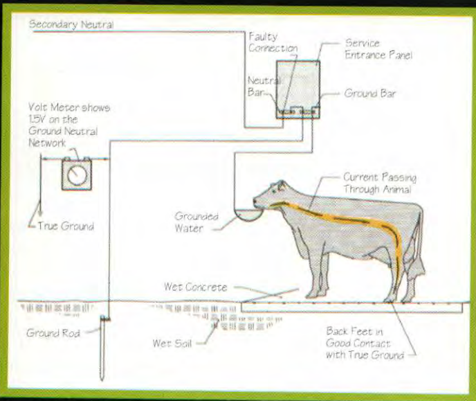
FIGURE 1 ONE EXAMPLE OF STRAY VOLTAGE 2
